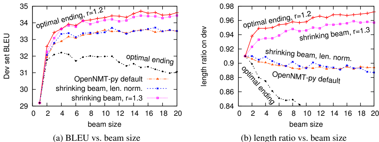
Figure 2: BLEU score and length ratio against beam size (on dev) of various beam search algorithms for neural machine translation.
