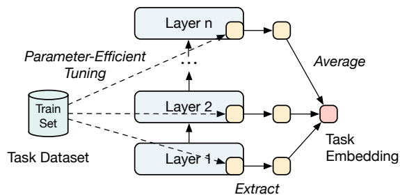
Figure 1: The workflow of using efficiently tuned parameters as task embeddings. The yellow boxes represent tunable parameters in Transformer layers.
