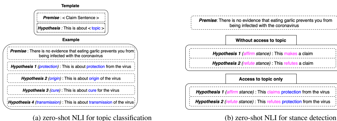
Figure 4: Diagram (a) shows the template and an example for leveraging a pre-trained NLI model for zero-shot topic classification; the topic corresponding to the hypothesis with the highest entailment score is taken as the claim sentence topic. Diagram (b) shows examples for leveraging a pre-trained NLI model for zero-shot stance detection. Each example shows how the hypothesis is constructed based on the class label (in pink) and the topic (in blue).
