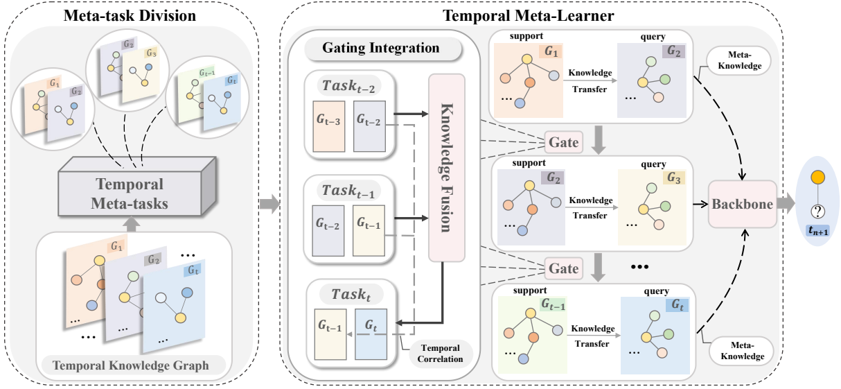
Figure 2: An illustration for MetaTKG. The TKG is firstly divided into many temporal meta-tasks (§4.1) for training. Then the Temporal meta-learner (§4.2) learns the evolutionary meta-knowledge from these tasks. Specially, according to the temporal characteristics of TKGs, we design a Gating Integration (§4.2.1) module to establish the temporal correlations among these tasks. During the learning process of each task, the knowledge gained from former ones will be fused and then transferred to the latter task. Finally, the obtained meta-knowledge from different tasks guides the backbone to learn to quickly adapt to new data for prediction over TKGs.
