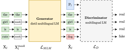
Figure 3: Discriminative source language prompt training with the generator being fine-tuned to generate \hat{X}_i from masked input X_i^{mask} whereas the prompt in the frozen discriminator (dashed) learns to discriminate real tokens from fake ones.
